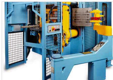
Quick Pattern Changer (QPC)
